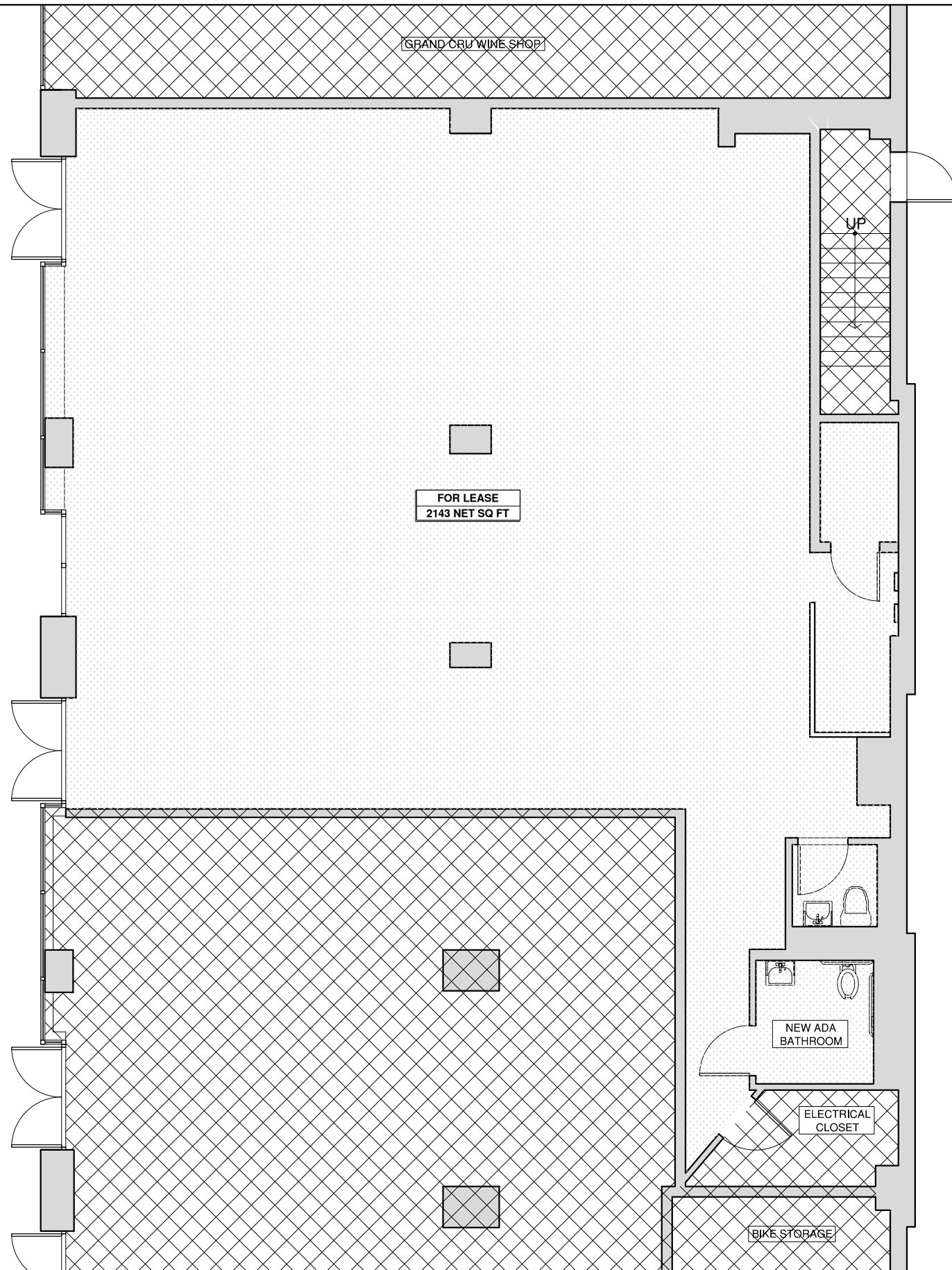
1 FIRST FLOOR VACANT RETAIL SPACE_POST REMOVAL PLAN SCALE: 1/8" = 1'-0"
